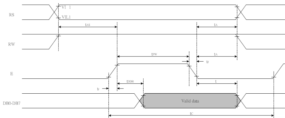
Write Mode (Writing data from MPU to ST7066U)
